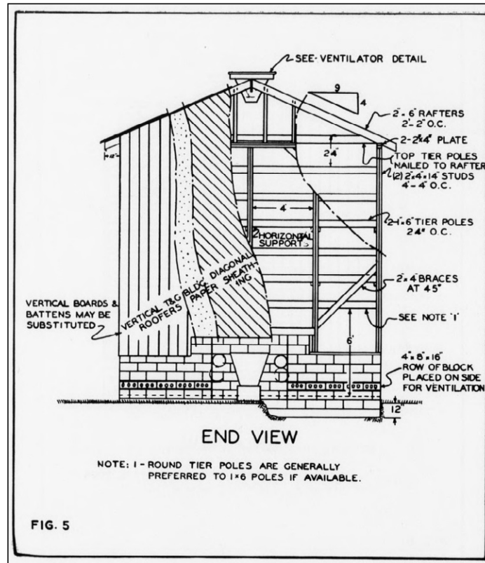
Figure 2.23: Illustration of concrete block, flue cured tobacco barn (Schaub 1953).
